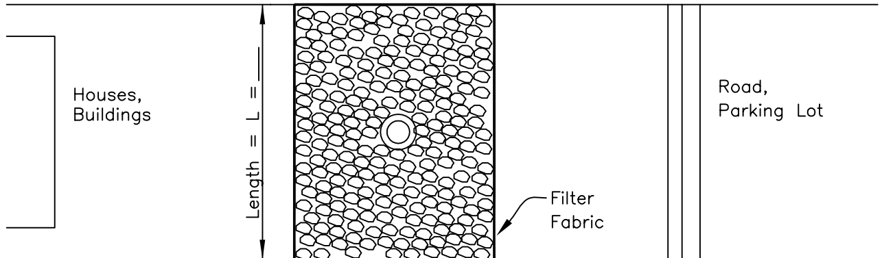
PLAN VIEW
