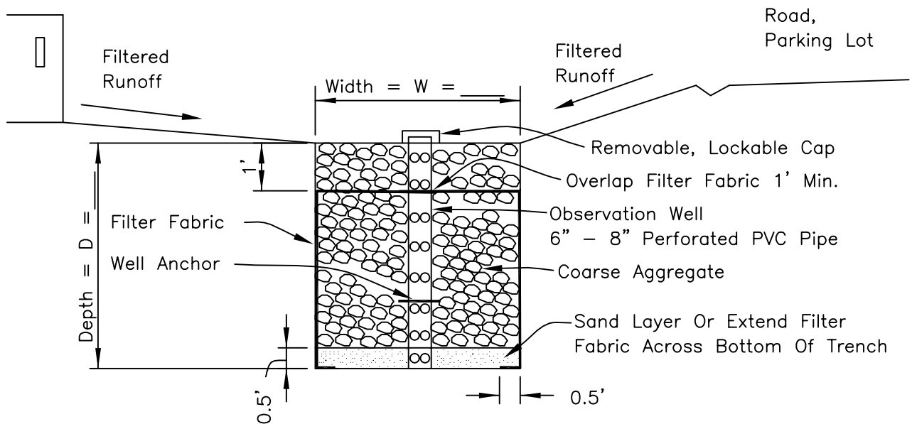
SECTION VIEW
