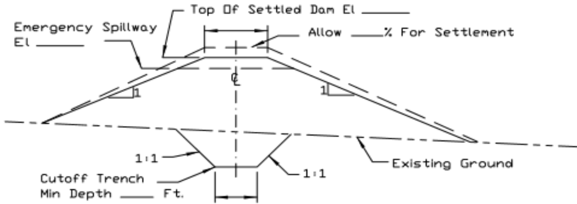
MAXIMUM CROSS SECTION OF DAM
