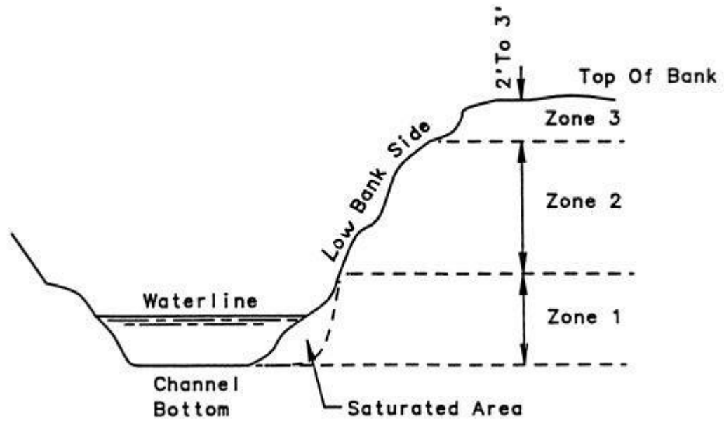
Figure 2 Plant Zones
