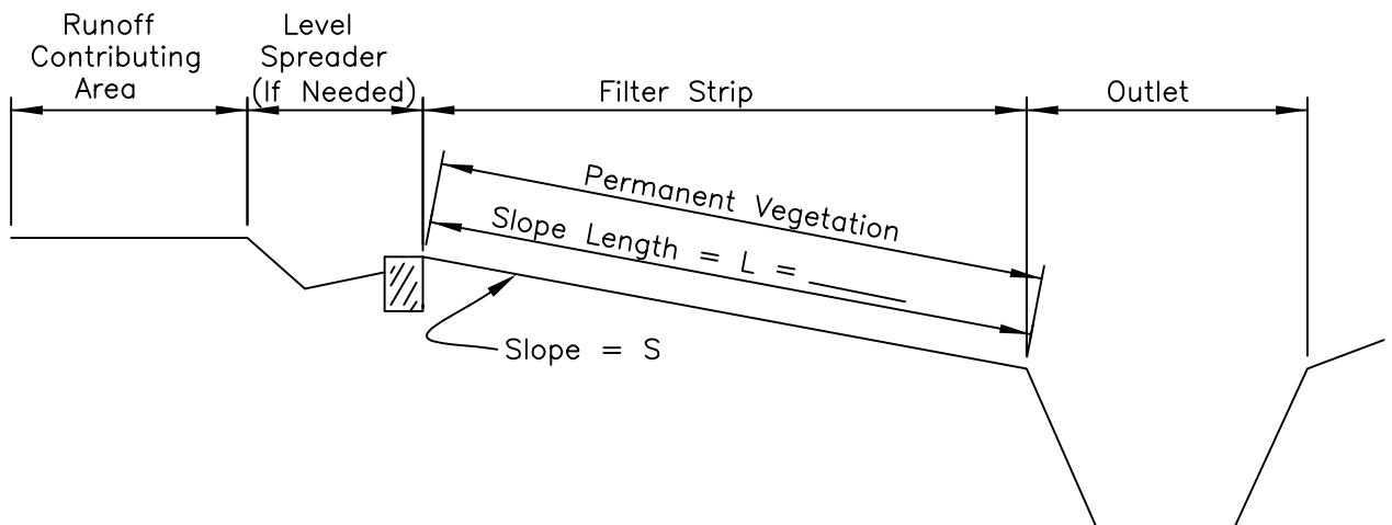
SECTION VIEW
