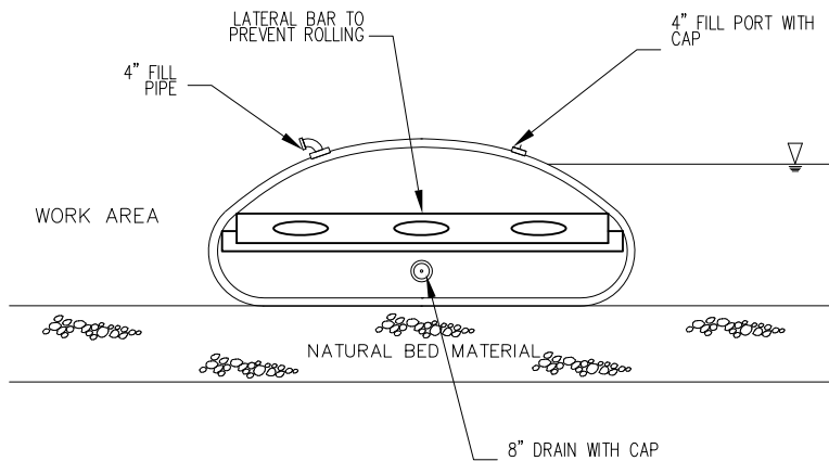
COFFERDAM PROFILE
